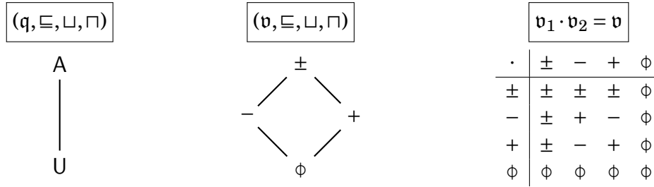
Figure 5.3: Syntax (iii): Qualifier constants, variances, and variance composition
