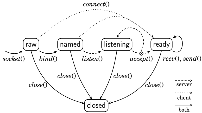
Figure 4.1: States and transitions for Berkeley sockets TCP
