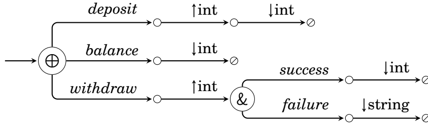
Figure 2.9: State diagram for ATM–bank protocol
