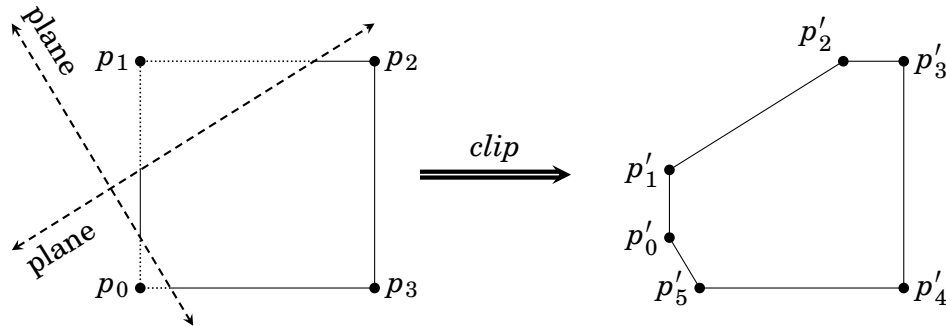
Figure 4.21: Example of polygon clipping
