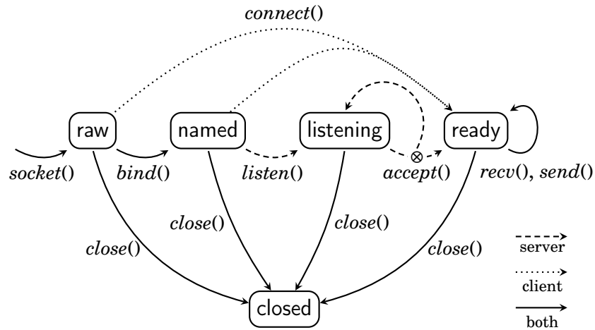
Figure 2.2: States and transitions for TCP (simplified)
