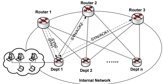
Figure 3. Sample network topology with asymmetric routing and multi-path routing.
