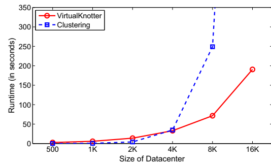
Fig. 7. Algorithm runtime overhead varying the size of a datacenter.
