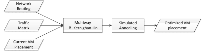
Fig. 4. Algorithm flowchart of VirtualKnotter. The diamond boxes are input/output data, and the rectangle boxes are functions.
