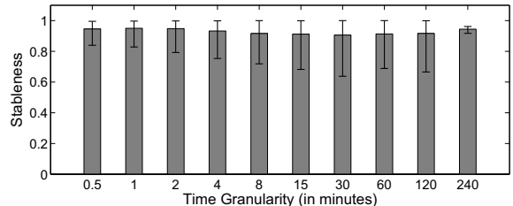
(b) Stableness indicator of core and aggregation links
