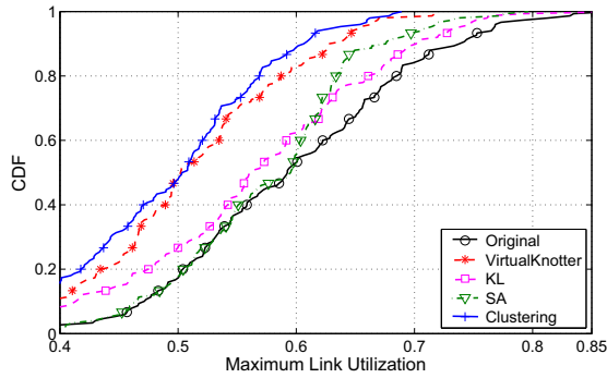
(b) CDF of MLU on Measurement-based Patterns (VM#=10K)
