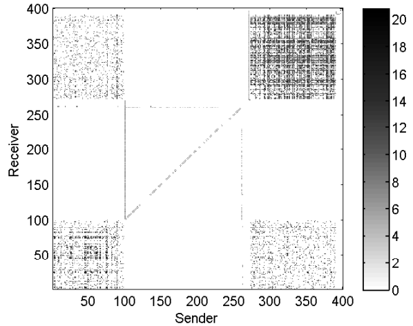
Fig. 1. An observed 30-sec traffic matrix. Each data point is the traffic volume from a sender (x axis) to a receiver (y axis). Gray scale reflects traffic volume in natural log of bytes.
