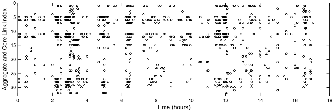
(a) Congestion timeseries before VirtualKnotter
