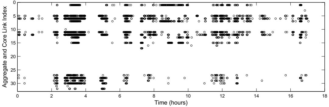
(a) Congestion timeseries before VirtualKnotter
