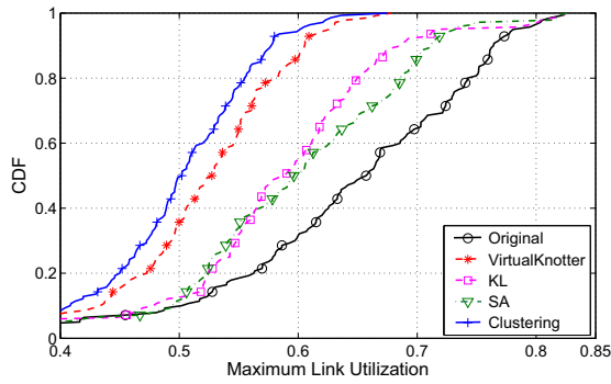
(a) CDF of MLU on Real-world Traces (VM#= 395)
