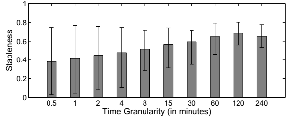
(a) Stableness indicator of pairwise traffic volume
