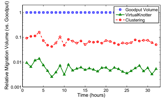
Fig. 6. Relative migration traffic compared with network goodput. The timescale is 30 minutes.
