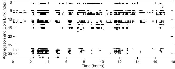
Fig. 2. Time and locations of congestion observed in the datacenter. Each circle represents a 30-second congestion occurred on a core or aggregation link.
