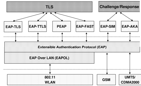
Figure 1: EAP protocols.
