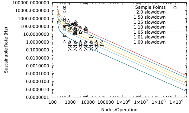
Figure 5: Possible rate and nodes (size) combinations given various constraints on application slowdown (NAS IS).
