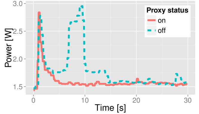
Fig. 2. Example power signatures during dwell time with and without JSSlow.
