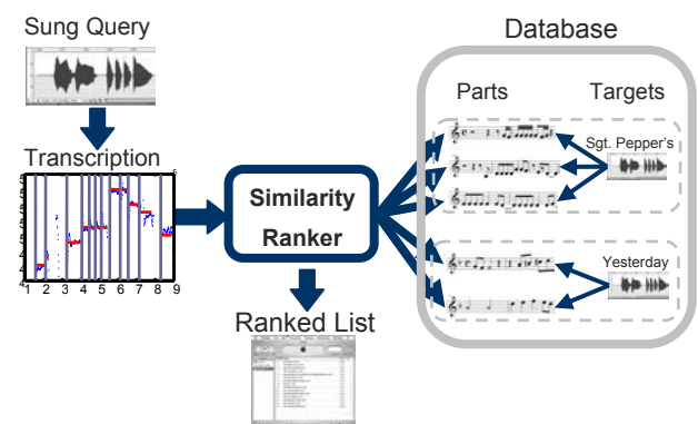
Figure 1. A typical Query-by-humming (QBH) system.
