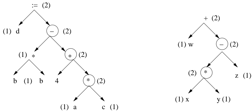
Figure 1: Problem 3. The children that are evaluated first are circled. All nodes are labeled by the minimum number of registers needed for the subtree rooted at them.
