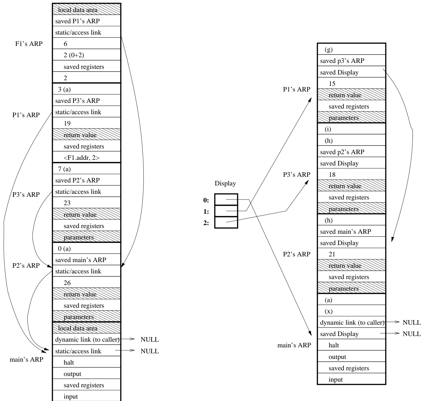
Figure 2: Problems 1 and 2. The shaded areas are there for reference and would not appear on the stack.
