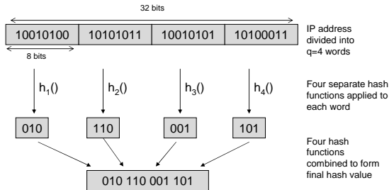
Figure 2: Modular hashing uses q hash functions to hash each word of the key, which are then combined for the final hash.
