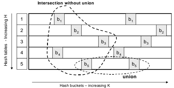
Figure 4: For two heavy changes, various possibilities exist for taking the intersection of each bucket's potential keys
